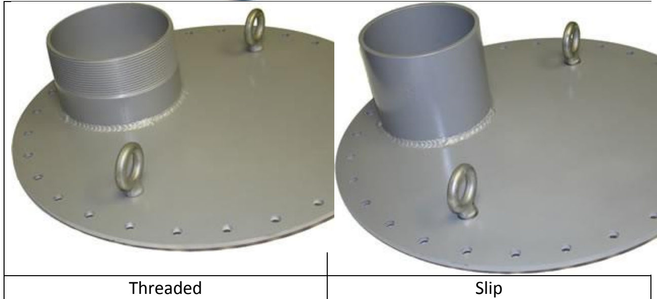
18"-30" Multi-Size Flow Diverter w/ Flanged End to accept Removable End Plates ( Threaded or Slip )
