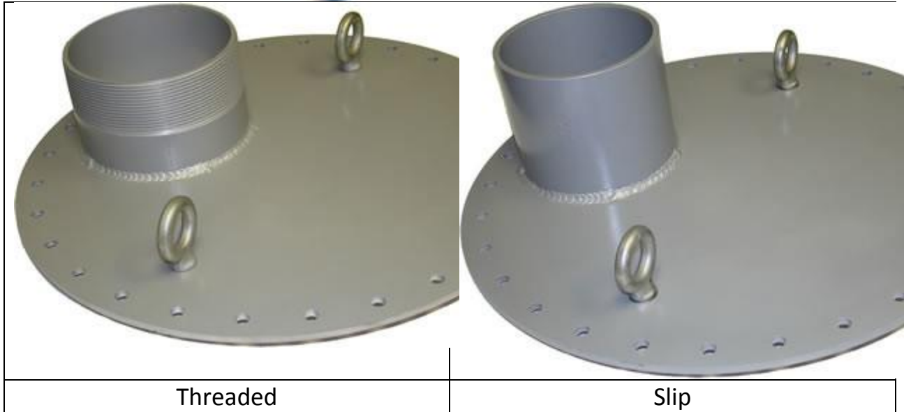
24"-36" Multi-Size Flow Diverter w/ Flanged End to accept Removable End Plates ( Threaded or Slip )
